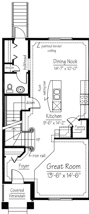
MAIN FLOOR PLAN
