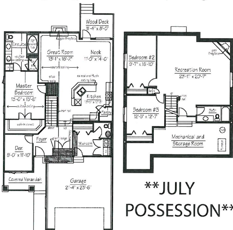
MAIN FLOOR PLAN 1504 sq. ft.
