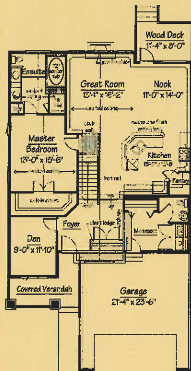
MAIN FLOOR PLAN 1504 sq. ft.
